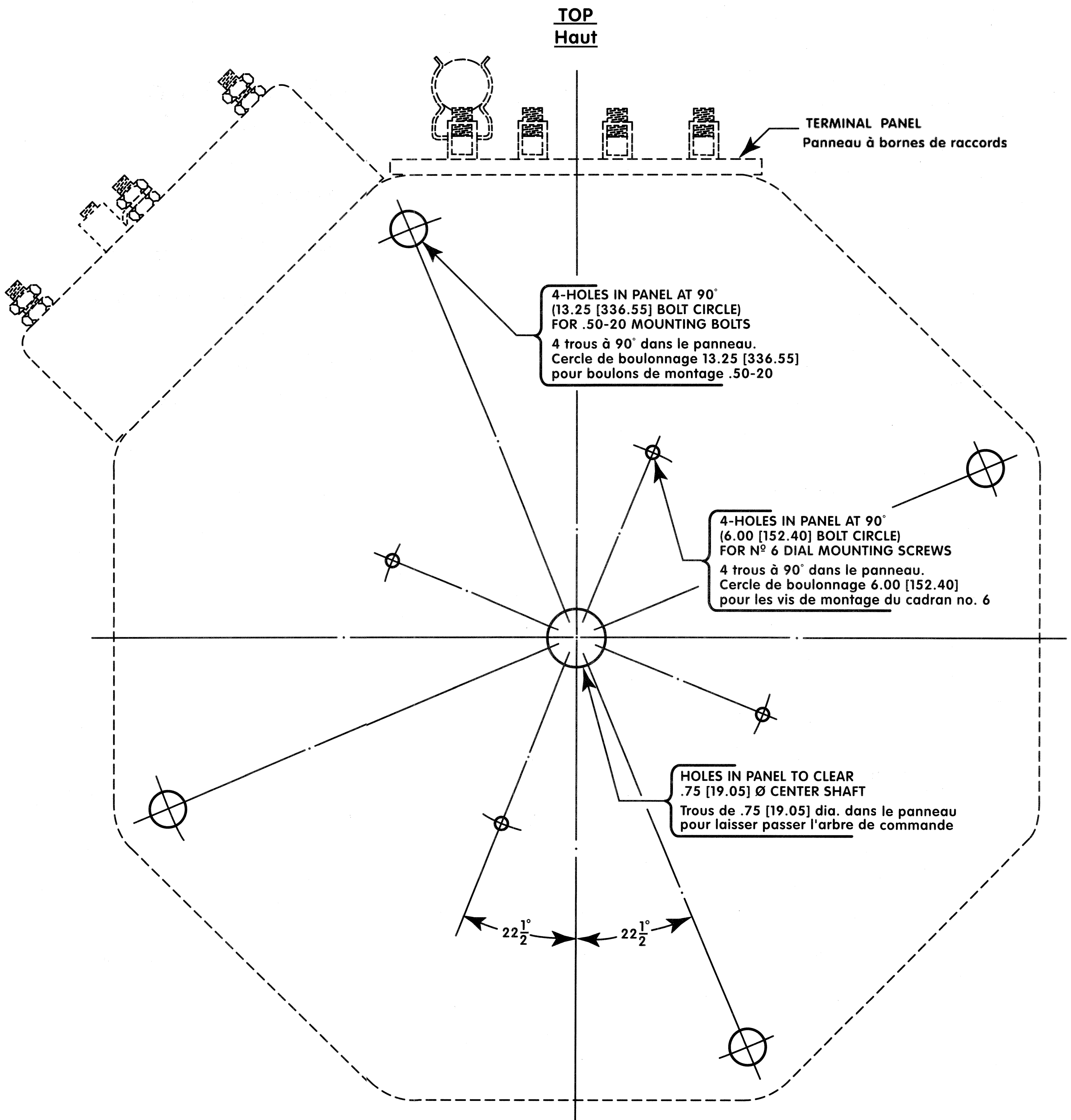
MOUNTING TEMPLATE Gabarit montage
