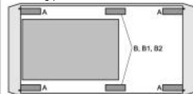
Mounting position horizontal-/ central rail
