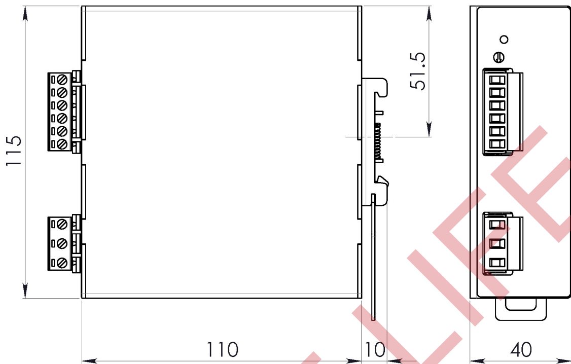
Figure 1. Mechanical Drawing
