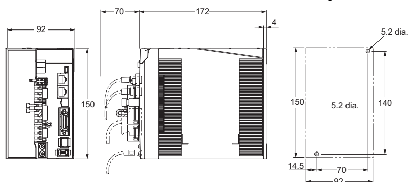
Mounting dimensions
