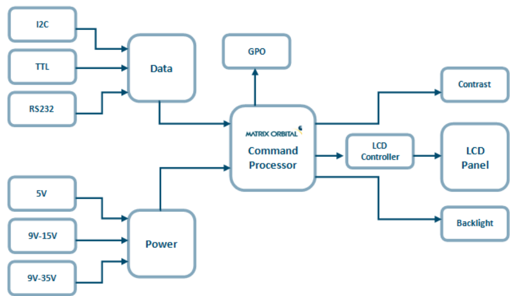
Figure 11: Functional Diagram
