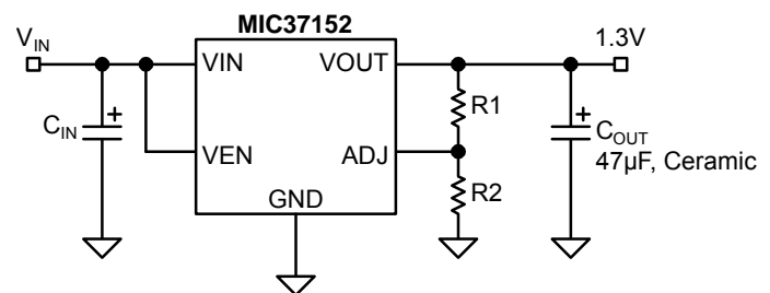
Adjustable Regulator
