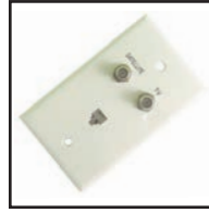
75-735-IV 75-735-W Satellite, TV wall plate built-in diplexer with TV ant., satellite and 4 conductor telephone jack. Available in ivory or white.
