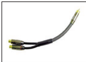
35-525-hg Shielded 8mm High Grade OFC "Y" cables with high quality gold plated connectors. RCA Male to dual RCA Females. 6" long. 35-525-hgm Same as HG Version only with Molded Connectors
