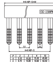
Dimensions - mm
