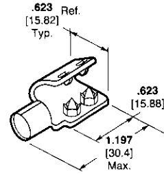
Type 11 Terminal
