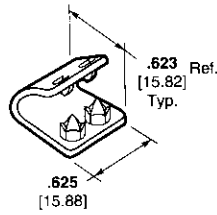
Type 10 Splice
