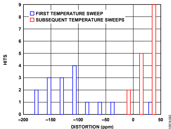
Figure 48. Thermal Hysteresis
