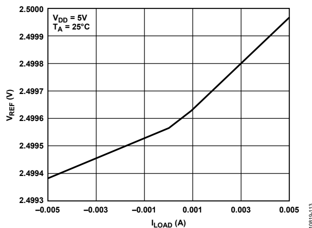
Figure 9. V_{REF} vs. Load Current ( I_{LOAD} )
