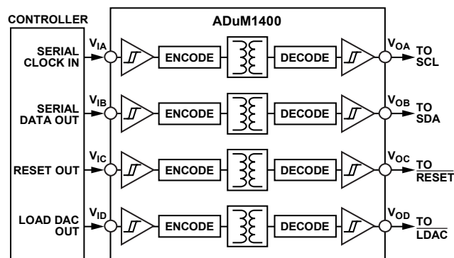
Figure 51. Isolated Interface
