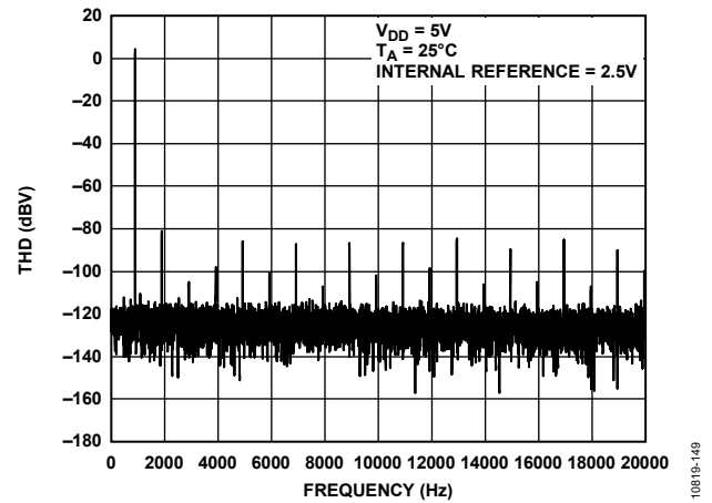
Figure 37. THD at 1 kHz
