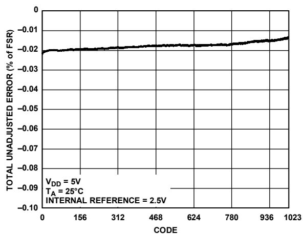
Figure 22. TUE vs. Code
