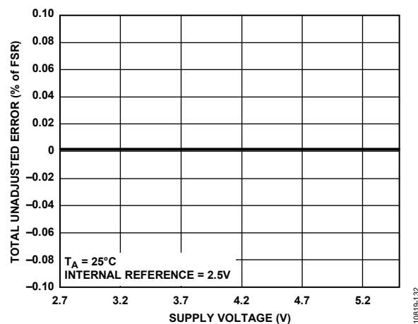
Figure 21. TUE vs. Supply Voltage, Gain = 1
