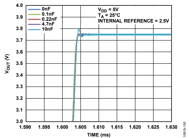
Figure 38. Settling Time at Various Capacitive Loads
