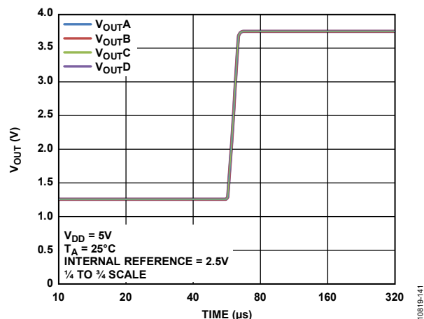
Figure 29. Settling Time
