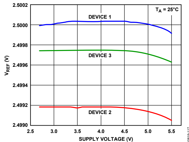
Figure 10. V_{REF} vs. Supply Voltage
