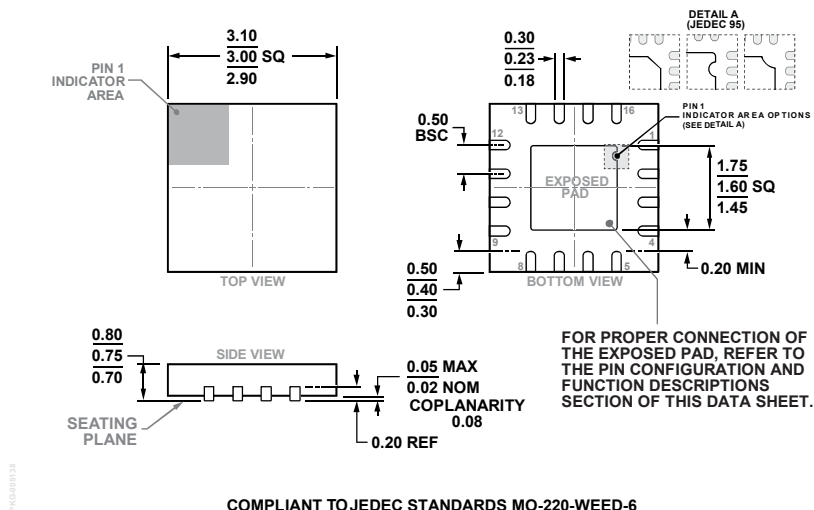
Figure 52. 16-Lead Lead Frame Chip Scale Package [LFCSP] 3 mm × 3 mm Body and 0.75 mm Package Height (CP-16-22)
