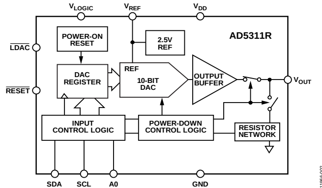
Figure 2. AD5311R
