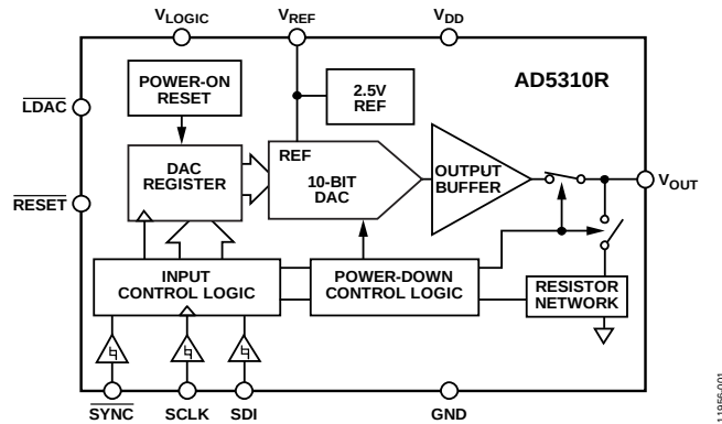
Figure 1. AD5310R
