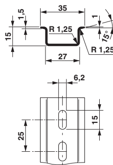
Dimensioned drawing
