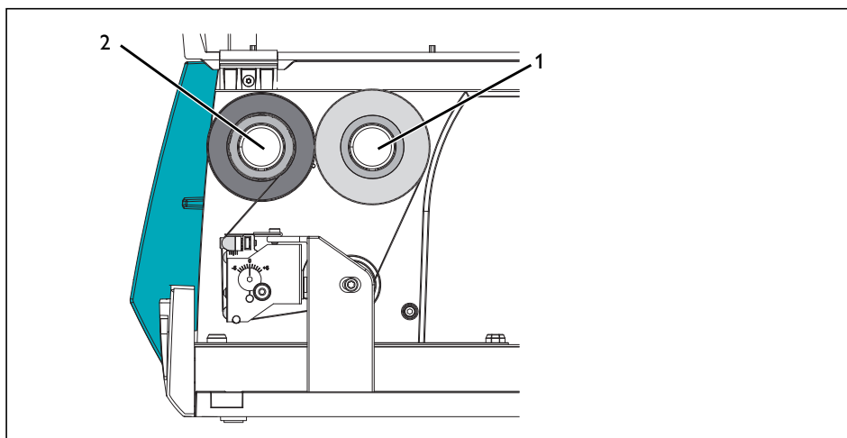
Figure 2-6 Feed path of the ink ribbon
