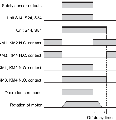
Timing chart
