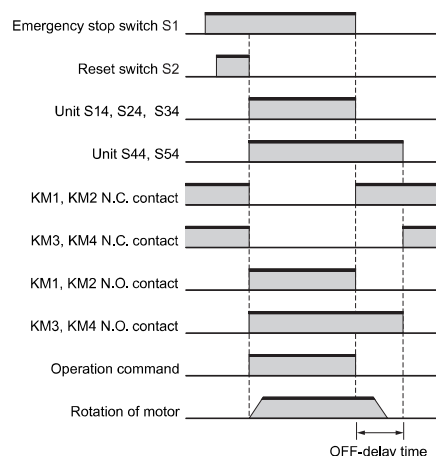
Timing chart
