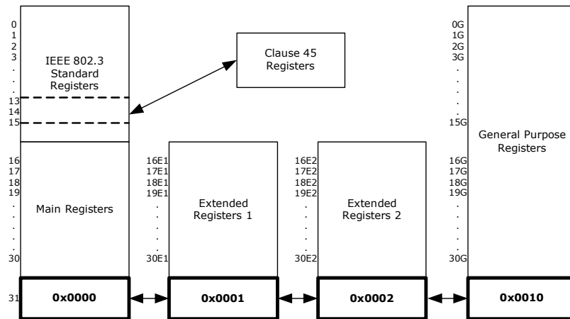
FIGURE 4-1: REGISTER SPACE DIAGRAM
