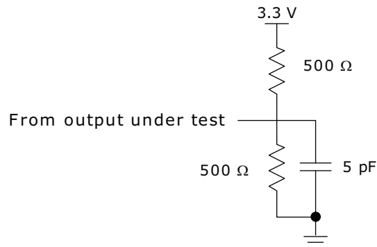
FIGURE 6-6: TEST CIRCUIT FOR TDO DISABLE TIME
