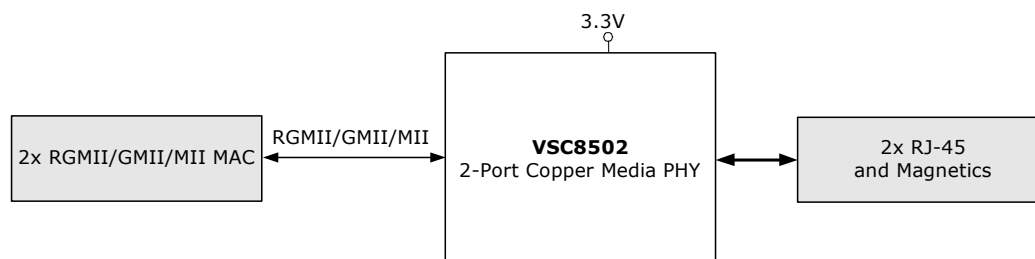
Copper Transceiver Application Diagram
