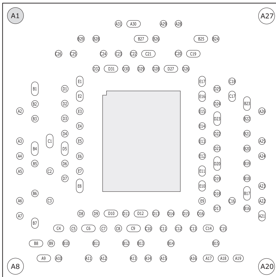
FIGURE 1-1: PIN DIAGRAM
