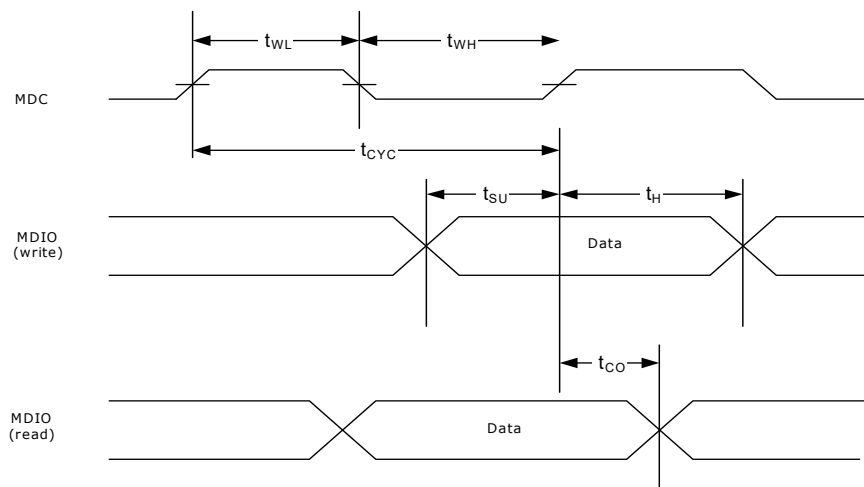
FIGURE 6-10: SERIAL MANAGEMENT INTERFACE TIMING
