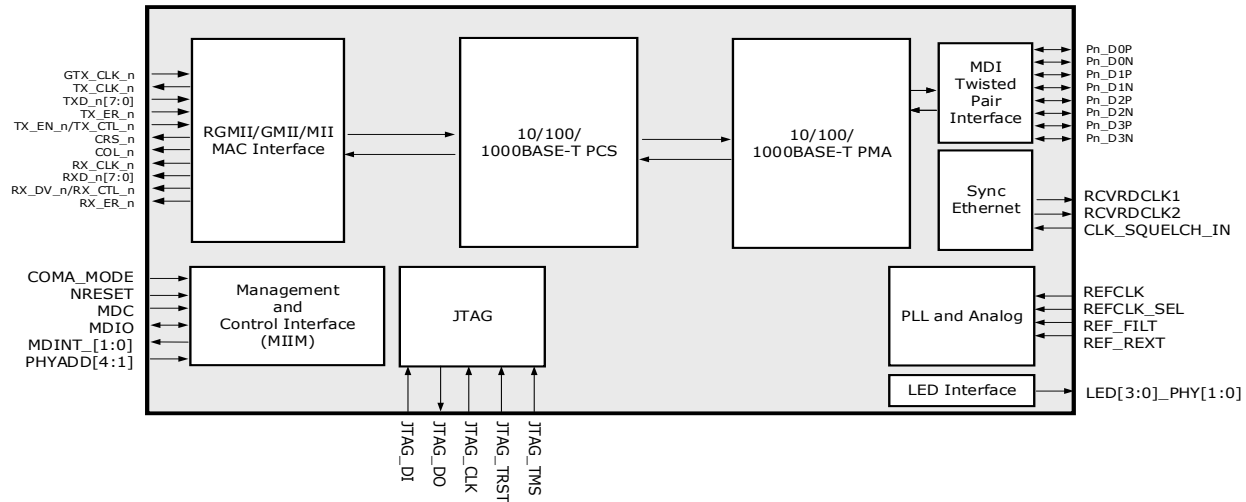
Block Diagram
