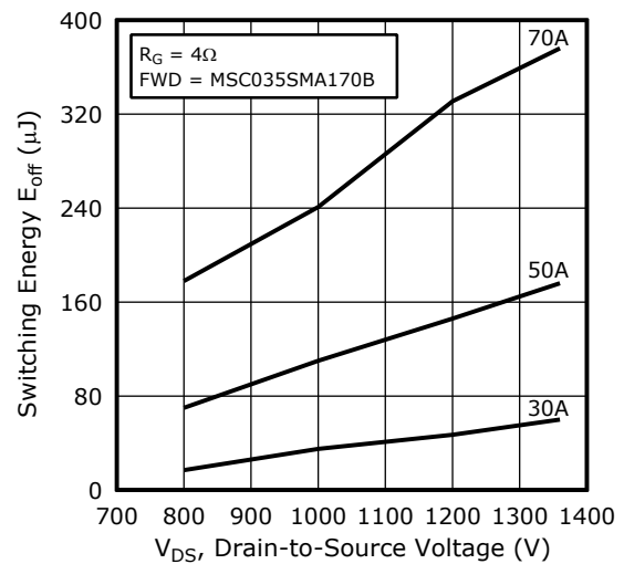
Figure 1-12. Switching Energy E_{off} vs. V_{DS} & I_D
