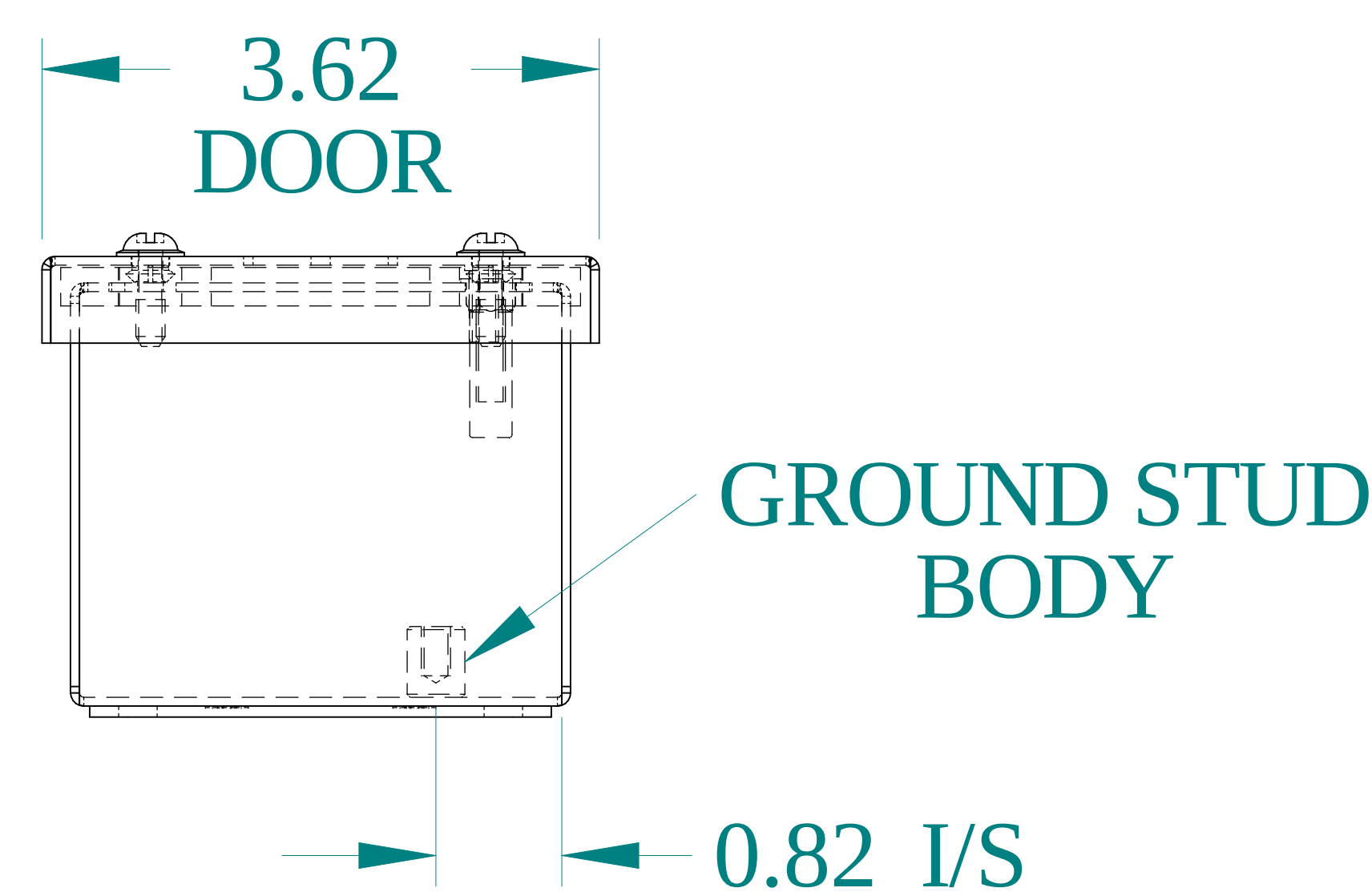
BOTTOM VIEW
