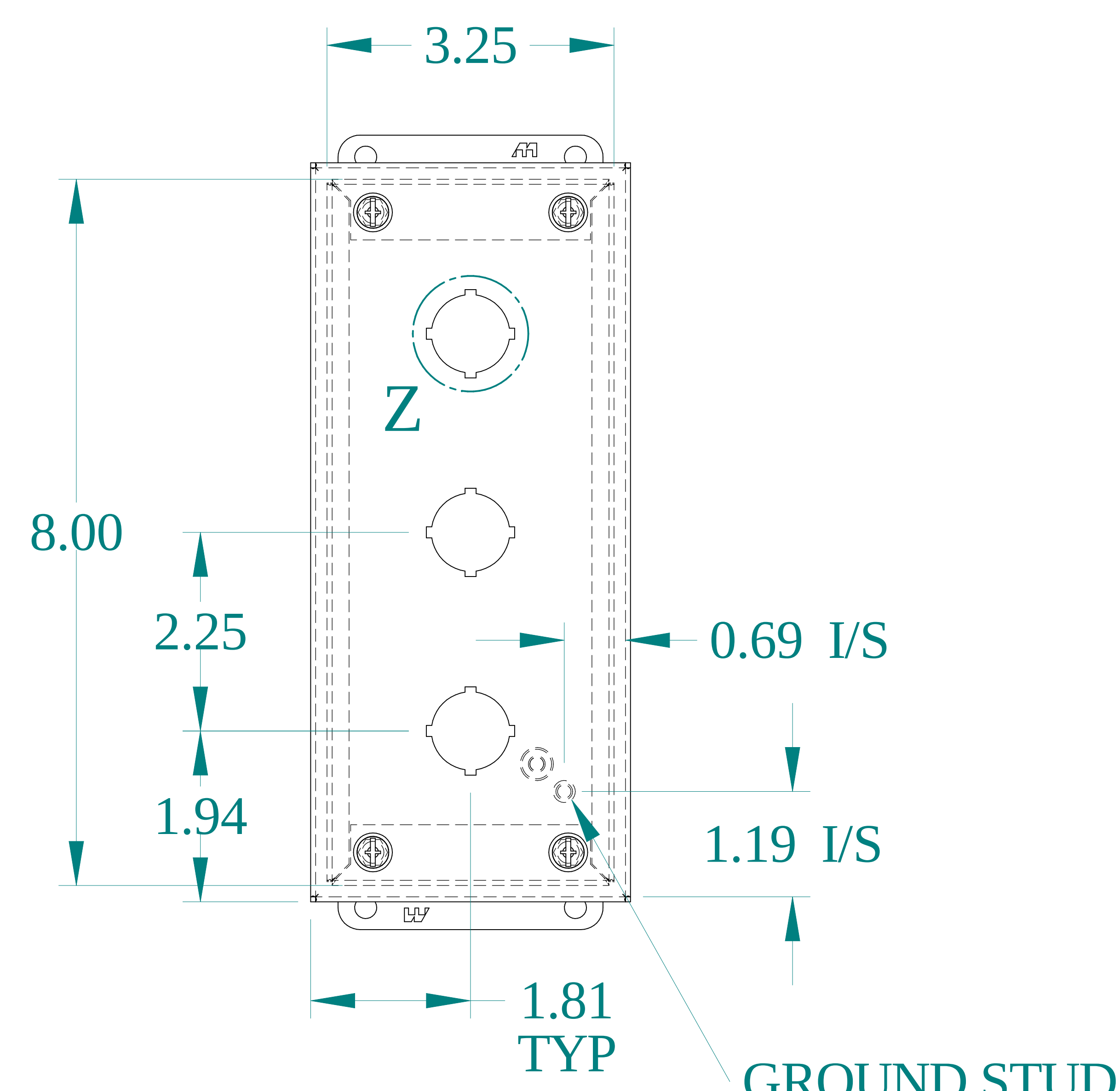
FRONT VIEW
