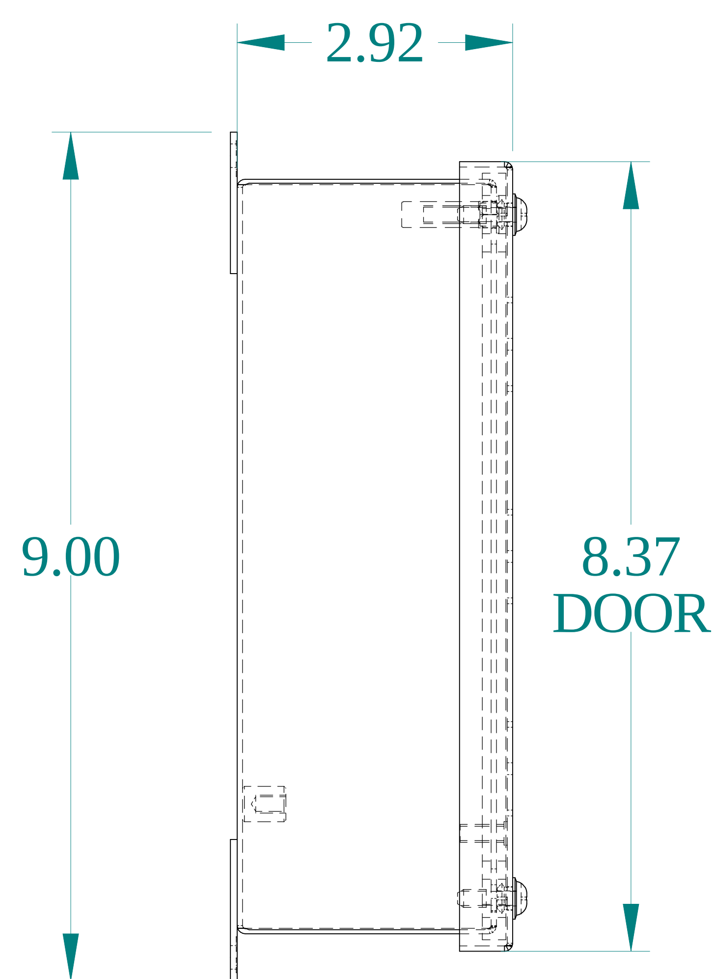
SIDE VIEW
