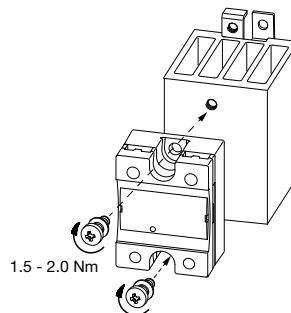
Fig. 12 Tighten screws alternately to 0.5 Nm and then continue to max. 2.0 Nm.
