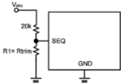
The SEQ pin can be used when master-slave power-supply tracking is required
