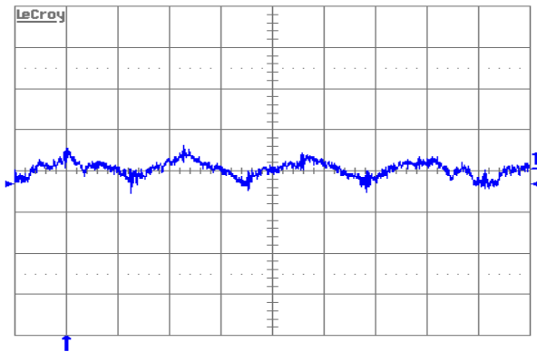
Figure 12. Input reflected-ripple current, i_s (10 mA/div.), measured through 10\ \mu\text{H} at the source at full rated load current and V_{in} = 48\text{V} . Refer to Figure 11 for test setup. Time scale: 1\ \mu\text{s}/\text{div} .
