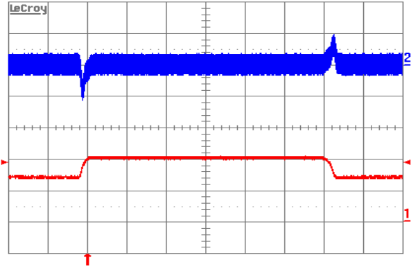
Figure 8. Output voltage response to load current step-change (6.5A–9.75A–6.5A) at V_{in}=48\text{V} . Top trace: output voltage (100 mV/div.). Bottom trace: load current (5A/div.). Current slew rate: 0.1A/ \mu\text{s} . C_o=1\mu\text{F} ceramic + 10 \mu\text{F} tantalum. Time scale: 0.2ms/div.
