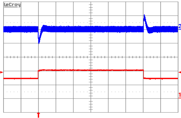
Figure 9. Output voltage response to load current step-change (6.5A–9.75A–6.5A) at V_{in}=48\text{V} . Top trace: output voltage (100 mV/div.). Bottom trace: load current (5A/div.). Current slew rate: 5A/ \mu\text{s} . C_o= 470\mu\text{F} POS + 1 \mu\text{F} ceramic. Time scale: 0.2 ms/div.
