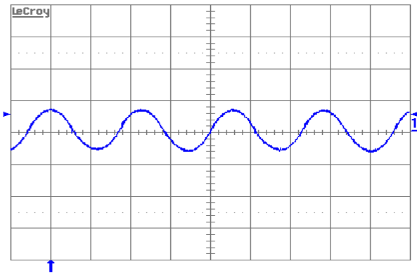
Figure 13. Input reflected ripple-current, i_c (200 mA/div.), measured at input terminals at full rated load current and V_{in} = 48\text{V} . Refer to Figure 11 for test setup. Time scale: 1\ \mu\text{s}/\text{div} .
