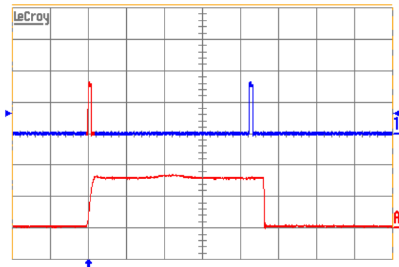
Figure 15. Load current (top trace, 10 A/div., 50 ms/div.) into a 10\text{m}\Omega short circuit during restart, at V_{in} = 48\text{V} . Bottom trace (10A/div., 1.0ms/div.) is an expansion of the on-time portion of the top trace.
