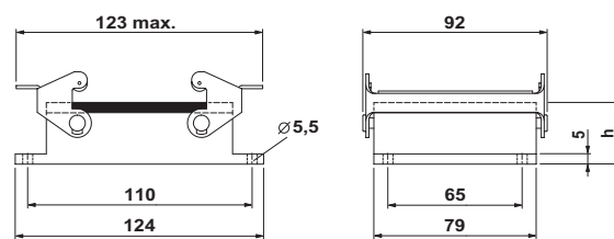
HC-B 32 AMQ...
