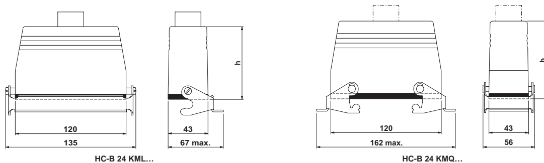
HC-B 24 KML...
