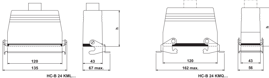
HC-B 24 KML...
