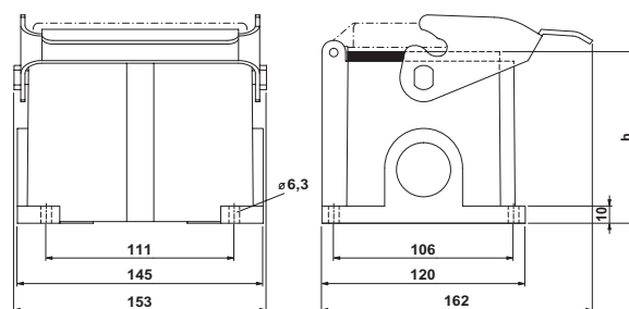
HC-B 48 SML...
