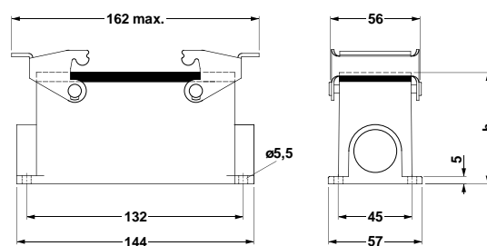
HC-B 24 SMQ...
