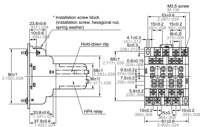
External dimensions
