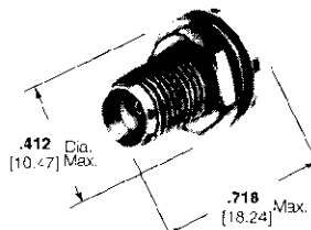
Brass body, nickel plated Part No. 228496-1
