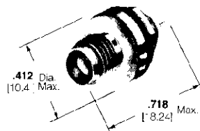
Brass body, nickel plated Part No. 228497-1
