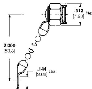
Brass, Nickel Plated Part No. 501368-1
