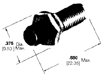
Part No. 221643-1
