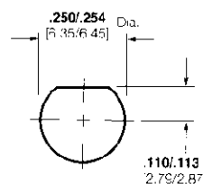
Recommended Panel Cutout for Bulkhead Jacks
