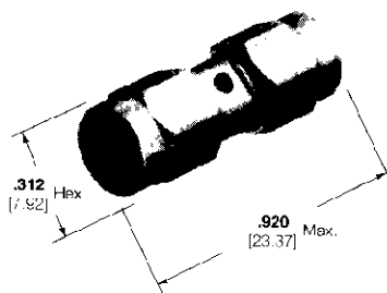
Part No. 221639-1
