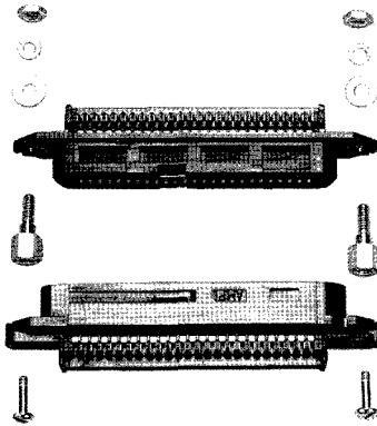
Screw Lock Hardware Kit Part Number 552568-1 (For rear panel mount applications, max. panel thickness shall be .062 [1.57].) (One kit required per assembly)
