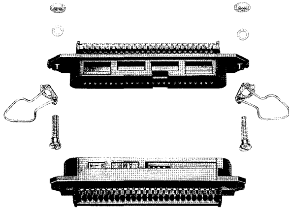
Bail Lock Hardware Kit Part Number 552567-1 (One kit required per assembly)
