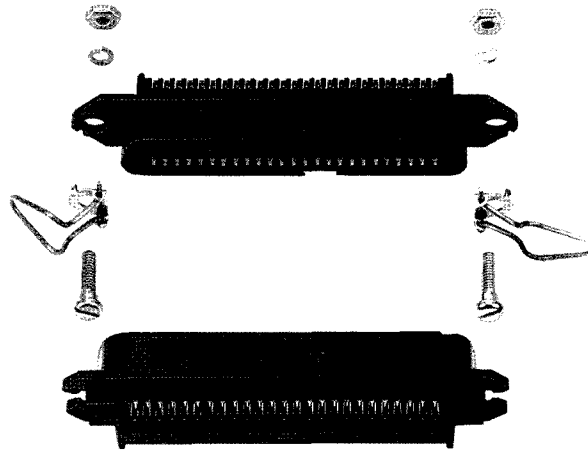
Bent Bail Lock Hardware Kit Part Number 552567-2 (For use with 90° strain relief cover—One kit required per assembly)
