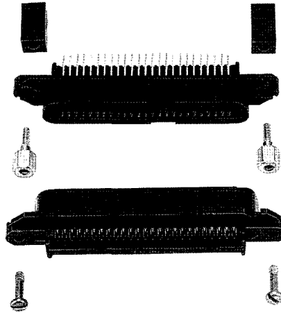
Screw Lock Hardware Kit—Part Number 552675-1 (One kit required per assembly)
