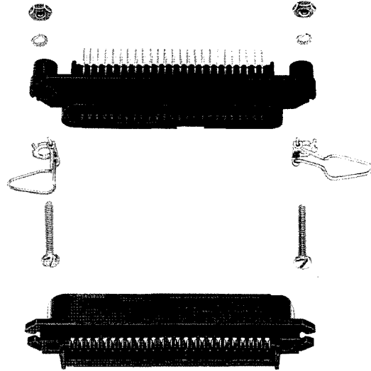
Bent Bail Lock Hardware Kit—Part Number 552562-2 (One kit required per assembly)
